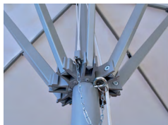
1. Lifting system "String"
